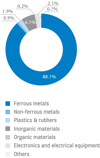
Material summary of a KONE MiniSpace™ unit
